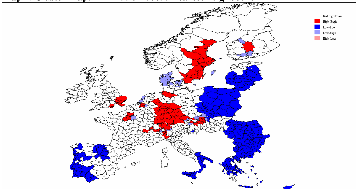
Map 4. Cluster map. IMR 1990-2006. 5 nearest neighbours
