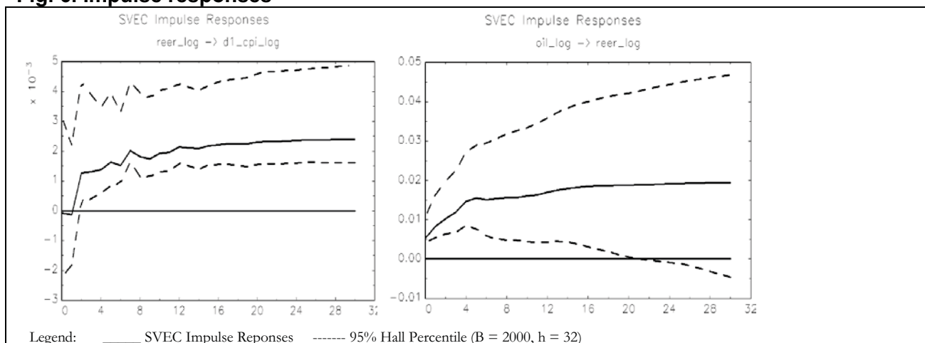
Fig. 6. Impulse responses
