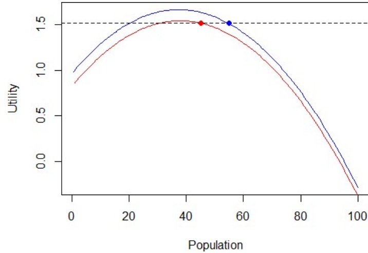
Figure 2: Two-region equilibrium.
