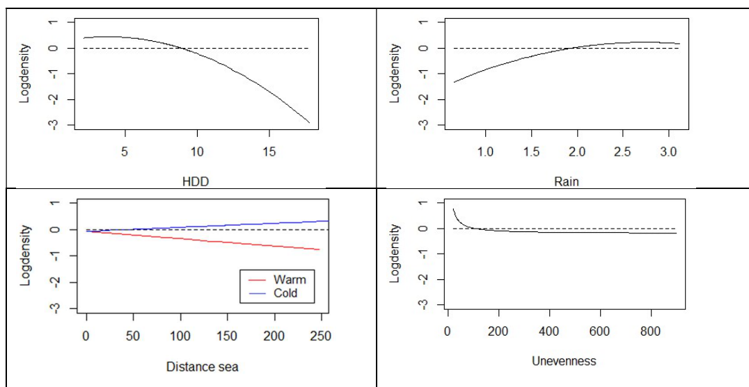
Figure 6. Partial dependence plots for non-binary variables.
