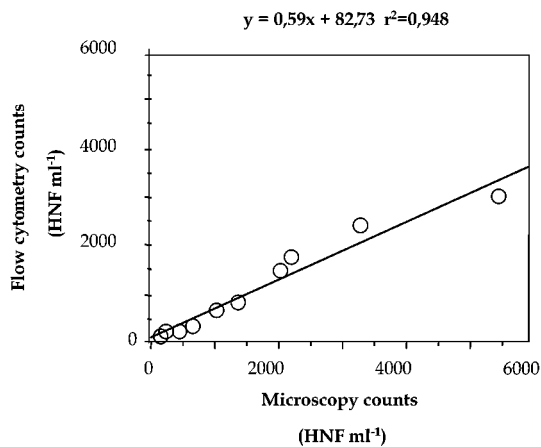
Fig. 7. Cross-calibration between epifluorescence microscopy and flow cytometry counts in a Rhynchomonas nasuta culture.
