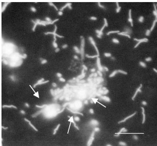
Fig. 8. Rhynchomonas nasuta attached to a bacterial aggregate. Scale bar: 10 \mu\text{m} .
