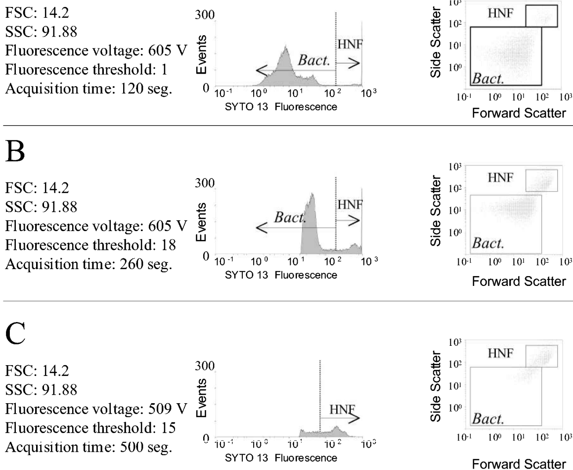
Fig. 3. Cytometric settings and the resulting cytometric detection of bacterioplankton and HNF applied to a seawater sample amended with an E. coli culture and incubated 66 hours. The same sample was analysed with the standard cytometric acquisition protocol for bacterioplankton (A), and with the new ones developed for a better detection of HNF in seawater (B and C). Cytometer settings are specified for each protocol. HNF: heterotrophic nanoflagellates, Bact. : bacteria.
