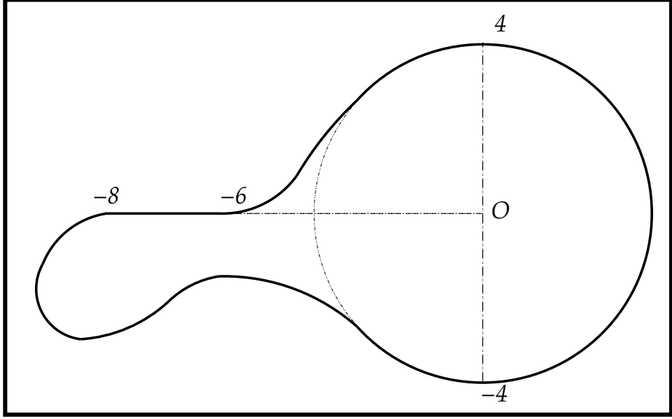
FIGURE A. The domain of Theorem 1.2.
