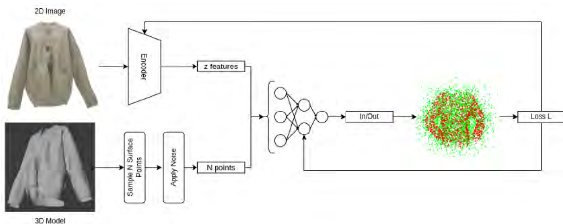
Figure 1. The foundational network architecture of our approach to 3D garment reconstruction
