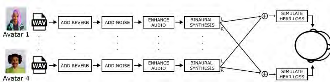
Figure 4. Signal flow in the proposed VR demo.
