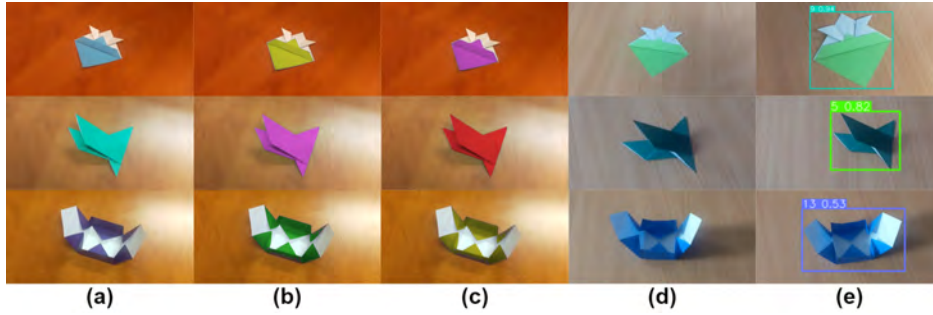
Figure 2. Example images for the samurai hat, bird and box origami models. Images from the train/val set with colour augmentation (a,b,c). Examples from the test set (d) and final detection (e).
